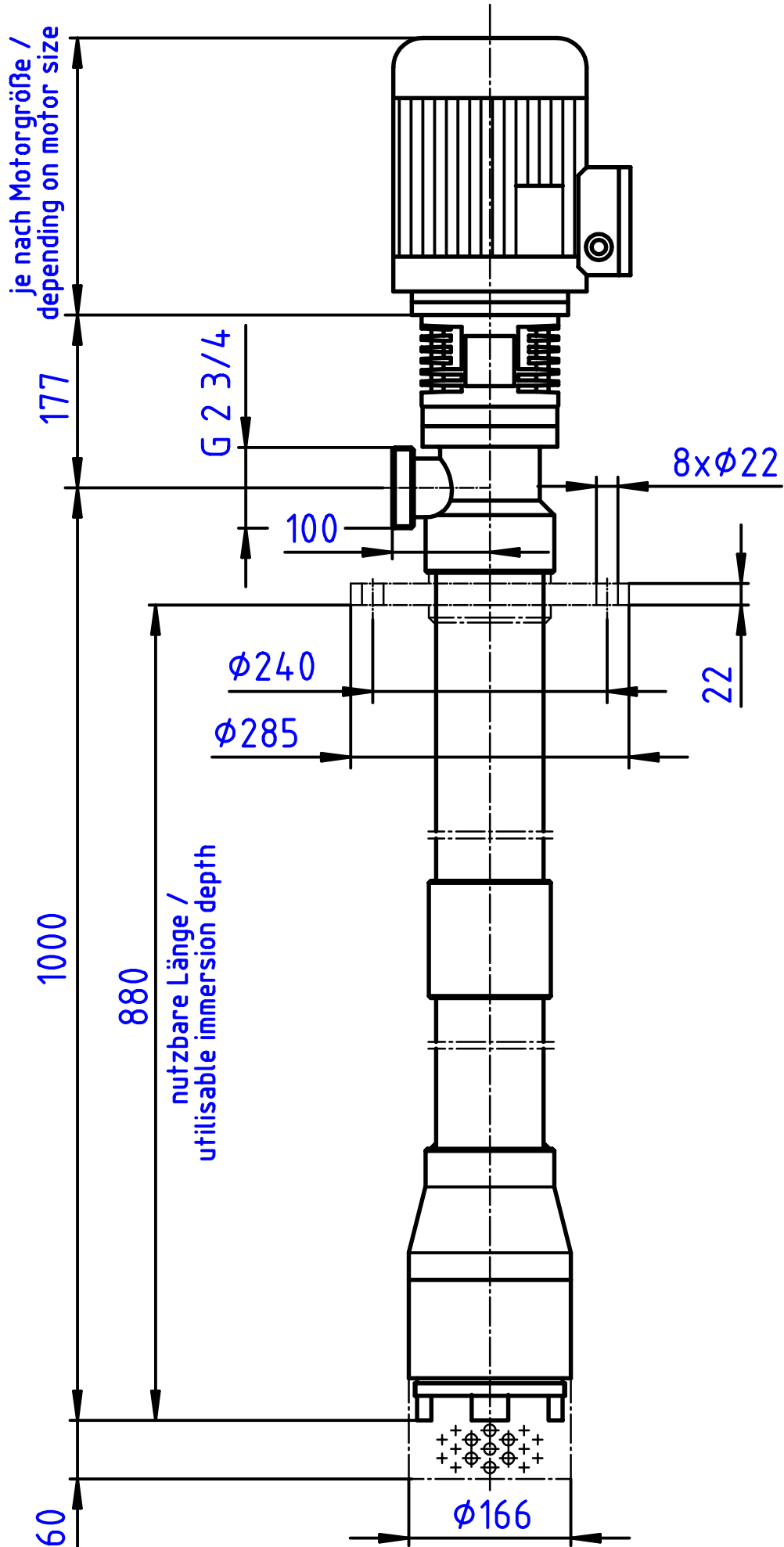
Tauchkreiselpumpe B6 PP Submersible centrifugal pump B6 PP
